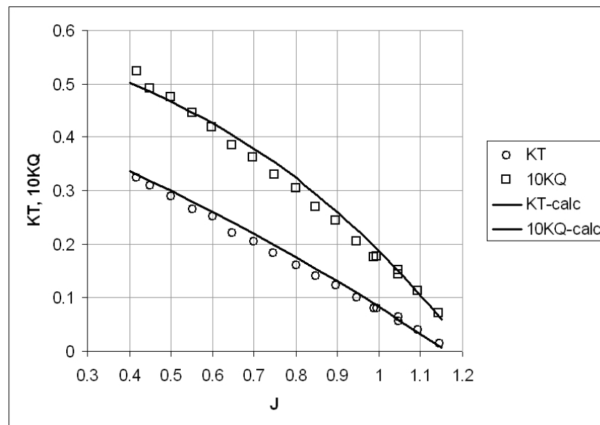
Open propeller performance (DTRC 4119)
