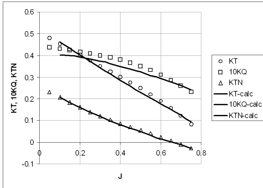
Ducted propeller performance (Kaplan 4.55 in 19A nozzle)
